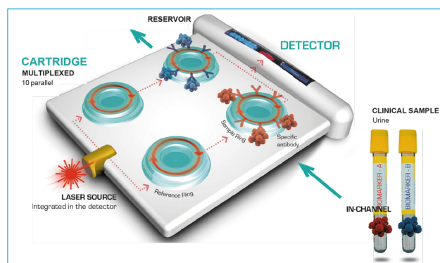
Fig.1 : Glass Laser Multiplexed Biosensor
